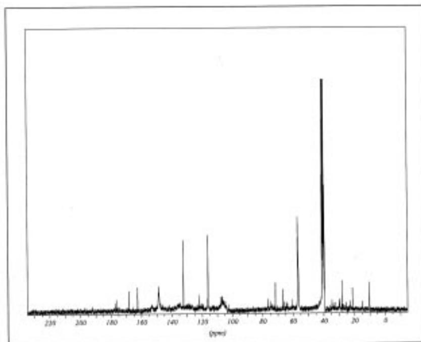
Figure 4 : ^{13}\text{C} -NMR spectrum for lignin precipitated by 20% v/v hydrochloric acid at \text{pH}_2
