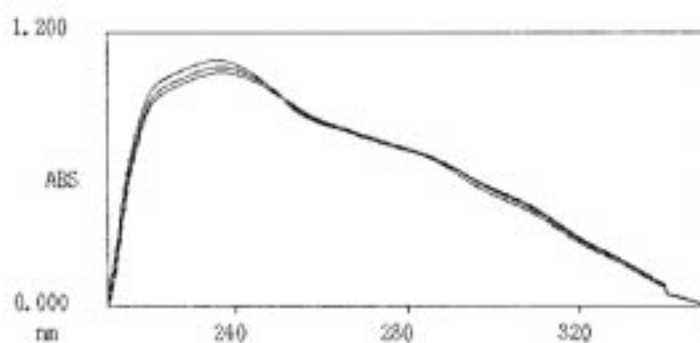
Figure 2 : Typical UV spectra of soda lignin precipitated from various concentrations of mineral acids
