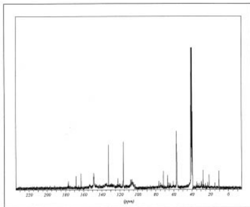
Figure 3 : C^{13} -NMR spectrum for lignin precipitated by 20% v/v sulfuric acid at pH_2
