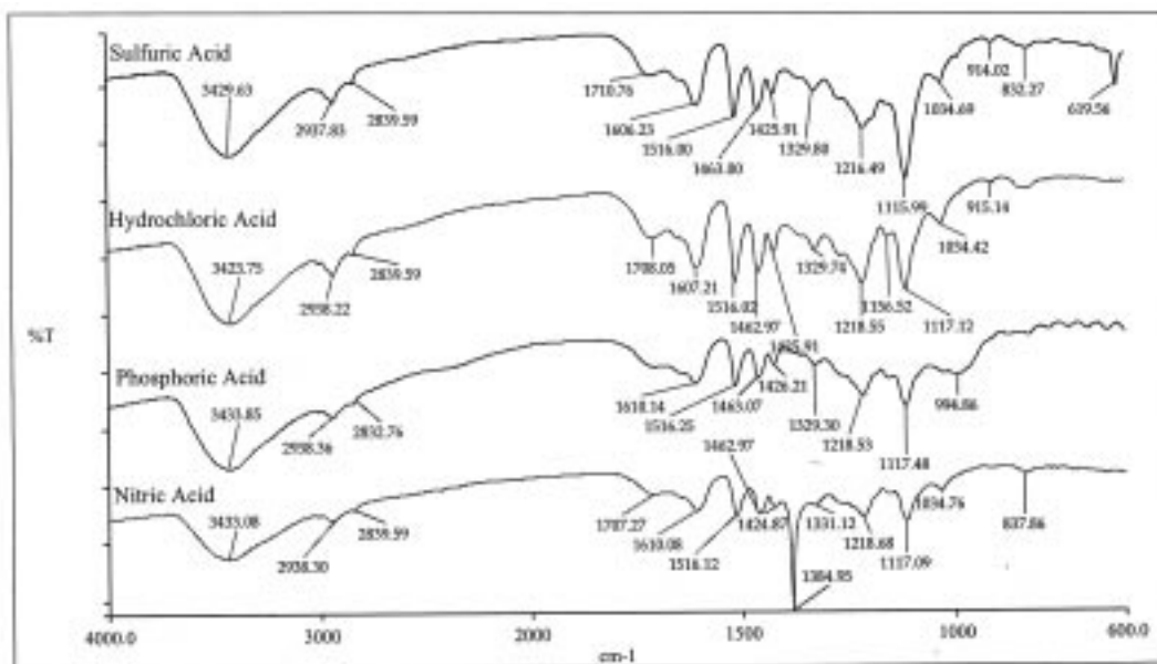
Figure 1 : Typical IR spectra of soda lignin precipitated from various mineral acids
