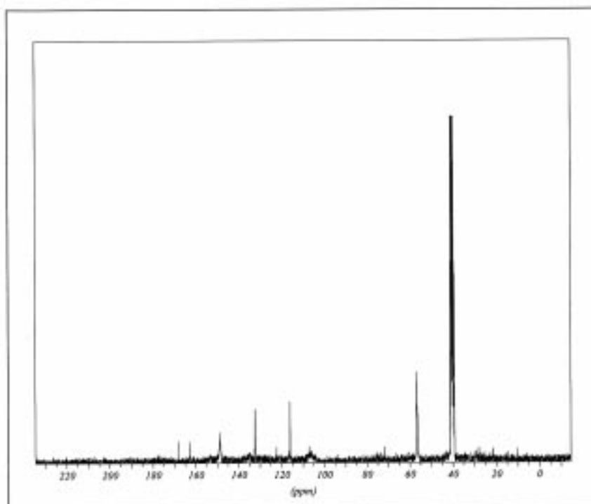
Figure 5 : ^{13}\text{C} -NMR spectrum for lignin precipitated by 20% v/v phosphoric acid at \text{pH}_2
