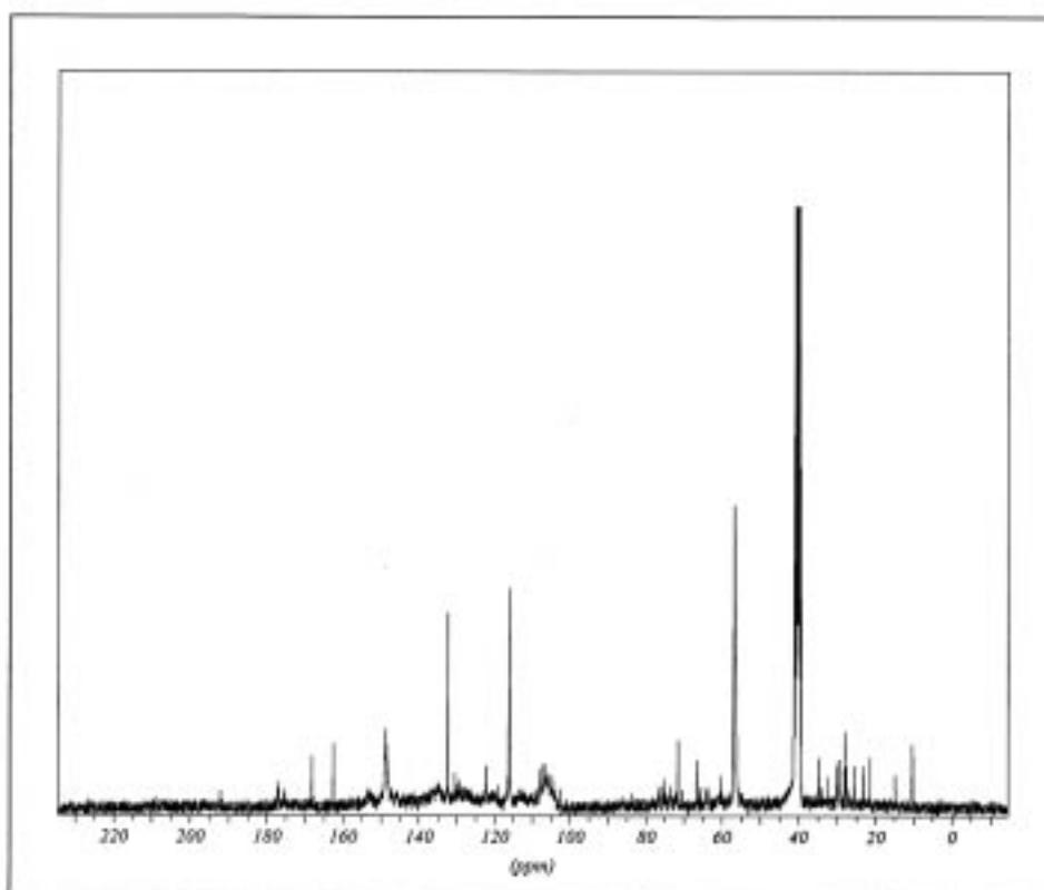
Figure 6 : C^{13} -NMR spectrum for lignin precipitated by 20% v/v nitric acid at pH_2
