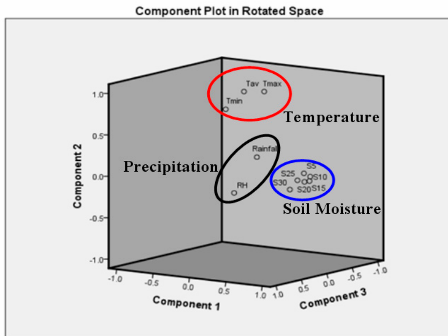
Figure 9 Grouping of climatic and soil moisture variables into 3 components of Precipitation , Temperature , and Soil Moisture using principle components analysis (PCA).
