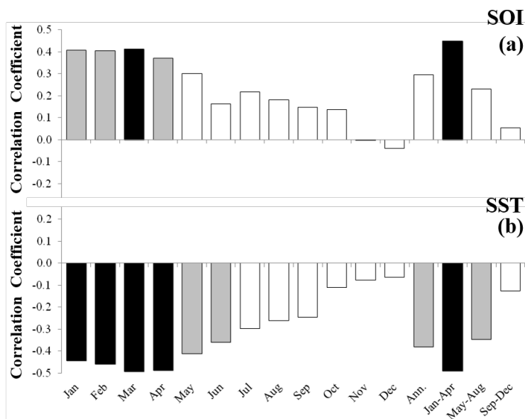
Figure 5 Plots of correlation coefficient ( r ) of ring width index with monthly, annual, and seasonal regional climate as a function of: (a) SOI and (b) SST. The grey bars represent a significant correlation ( p < 0.05 ), while black bars represent a highly significant correlation ( p < 0.01 ).
