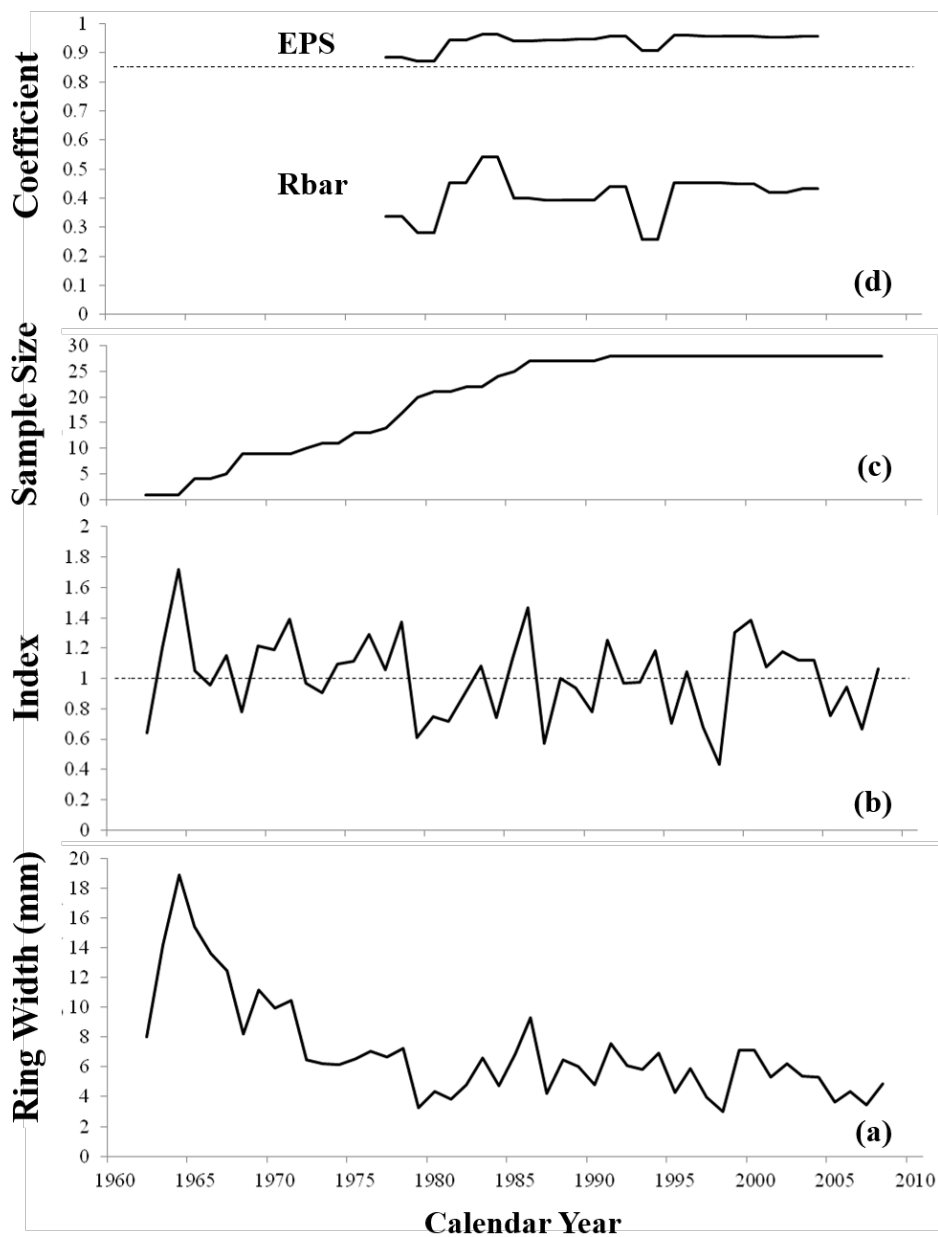
Figure 3 Teak annual ring plots: (a) mean annual ring width, (b) annual ring width index, (c) sample size, and (d) running EPS and Rbar.
