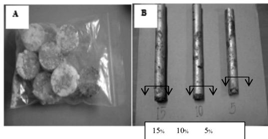
Figure 1. Photographs of the pressed composite mixture before sintering (A) and the casted sand composites with alumina of 5, 10, and 15 wt% (B).
