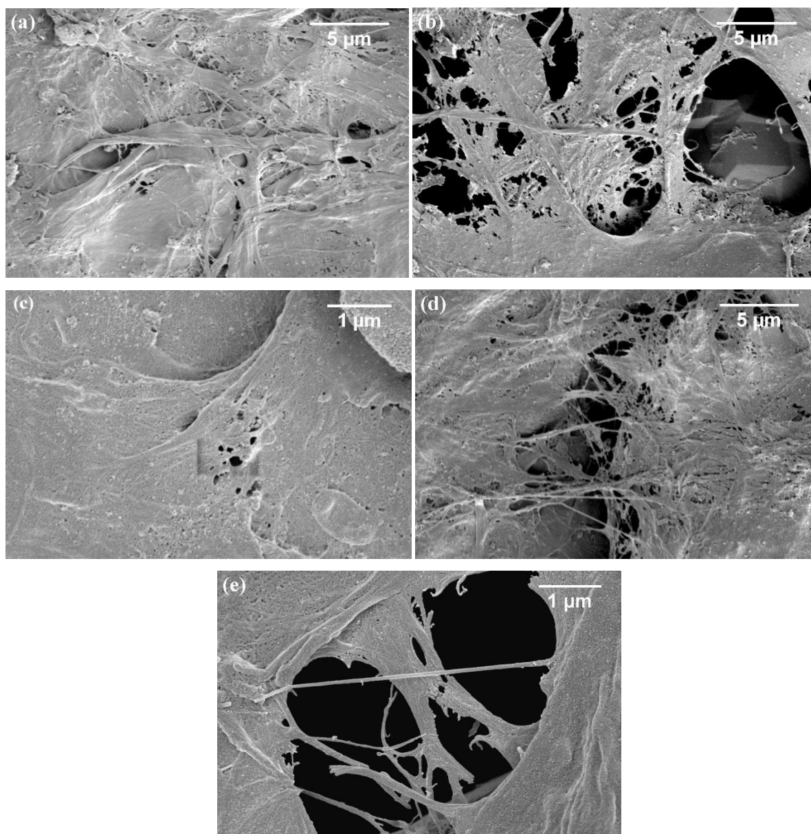
Figure 4. FE-SEM images of cellulose fibers prepared by mechanically homogenizing: (a) the bleach cellulose; and the hydrolyzed cellulose obtained by hydrothermal hydrolysis with (b) 0% OX; (c) 5% OX; (d) 10%OX and (e) 30%OX.
