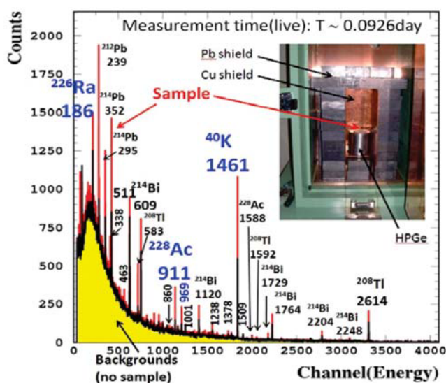
Figure 3. \gamma -ray spectra of LUSI soil sample and background measured with 526 \text{cm}^3 HPGe detector.
