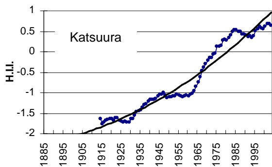
Fig. 2 H.I.I. for Tokyo with respect to Mito, Kumagaya, Choshi, Maebashi and Katsuura.
