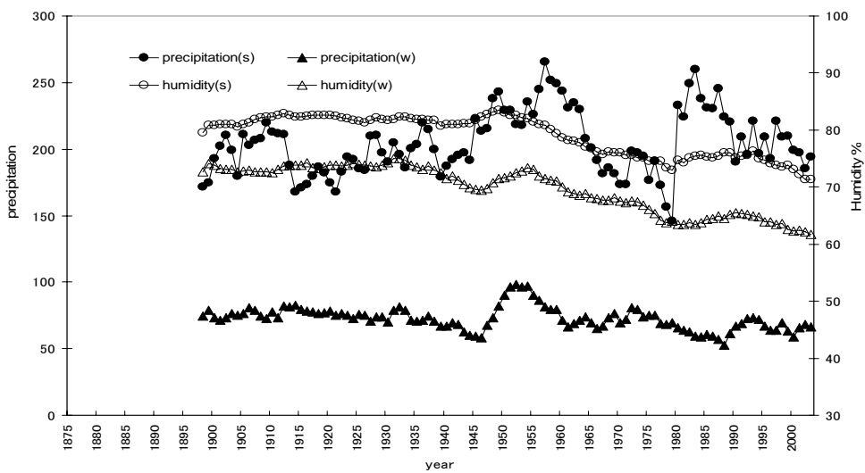
Fig. 1 Triangulated average trend of precipitation and humidity profile (Summer and Winter) of Tokyo, Sendai and Fukuoka.
