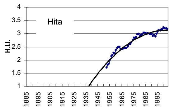
Fig. 3 H.I.I. for Sendai (with respect to Miyako and Ishinomaki) and Fukuoka (with respect to Saga, Iizuka and Hita).
