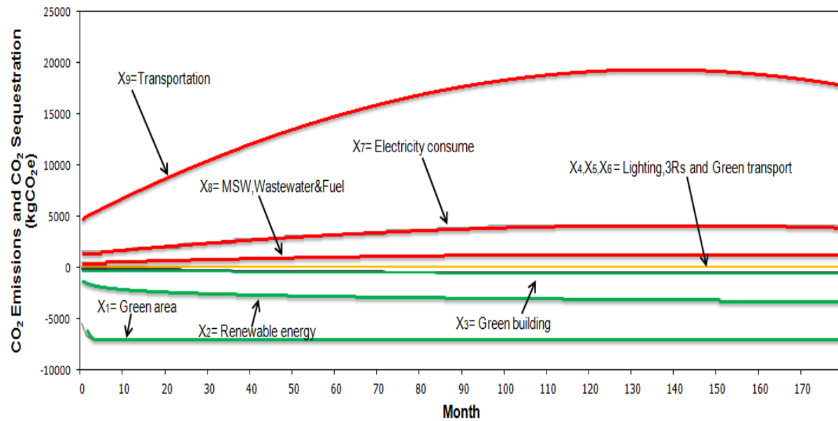
Figure 5 \text{CO}_2 emissions and \text{CO}_2 sequestrations of BAU
