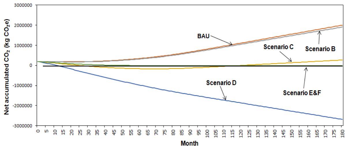
Figure 6 The net accumulated \text{CO}_2 e graph of scenario A, B, C, D, E and F
