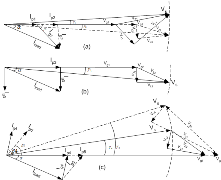
Figure 2 Phasor diagram for current from GCPV system. (a) GCPV current is less than load current (b) GCPV current is equal to load current (c) GCPV current is greater than load current.
