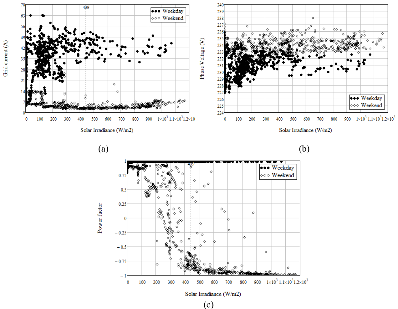
Figure 3. Condition of grid during weekday and weekend (a) Grid Current (b) Phase Voltage (c) Power factor.
