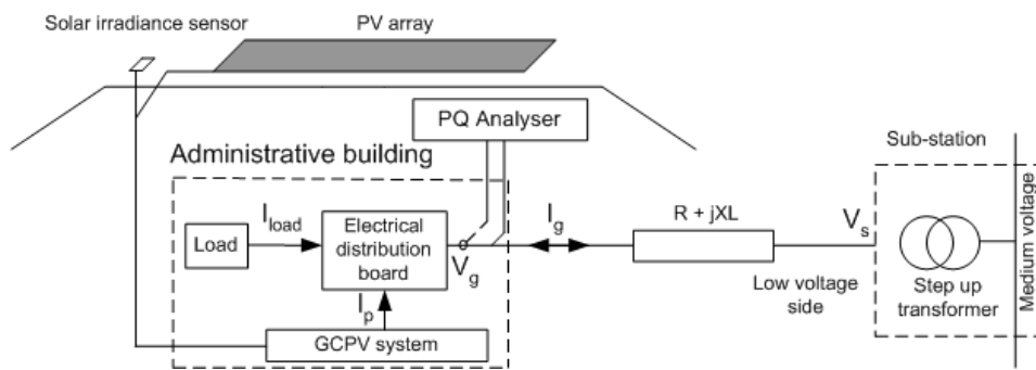
Figure 1. Model for GCPV system with direction of current flow
