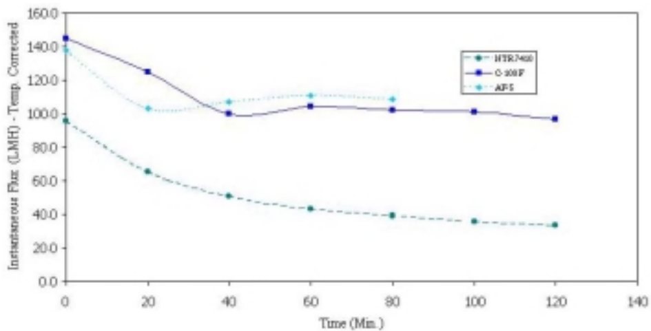
Figure 5. Flux performance for test membranes
