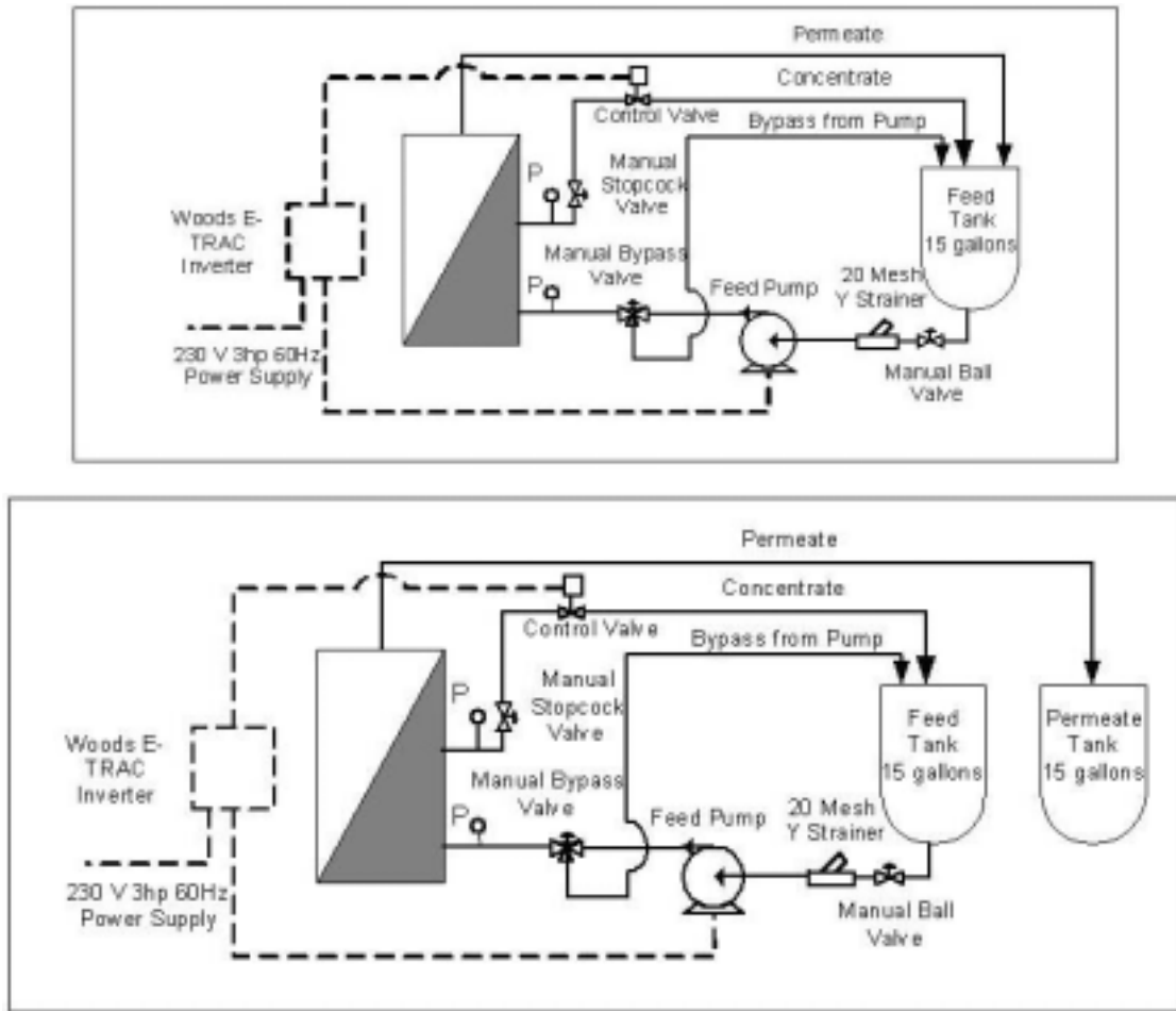
Figure 4. Pilot test schematic a) Initial, b) Batch circulation
