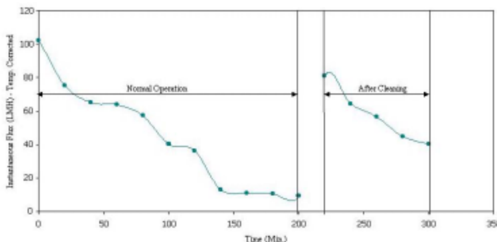
Figure 6. Flux and cleaning performance for NTR-7450 membrane
