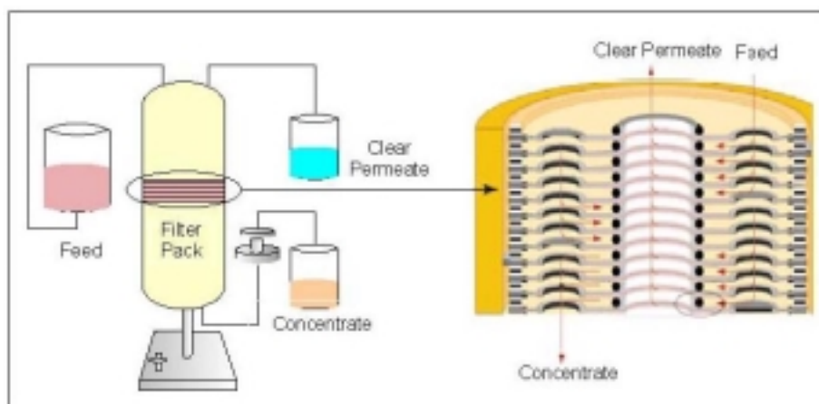
Figure 3. Inside look at the VSEP plate and frame assembly
