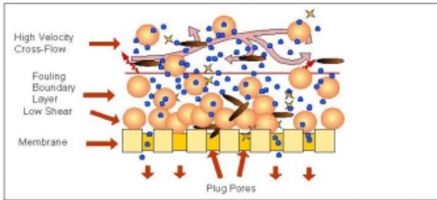
Figure 1. Conventional cross-flow filtration
