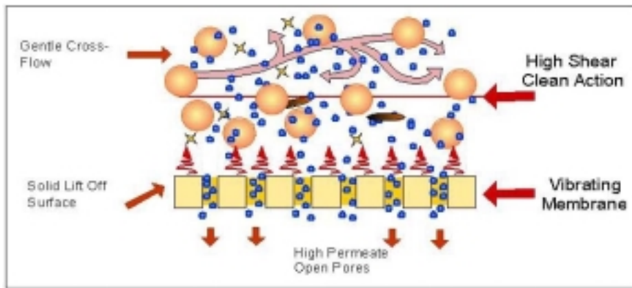
Figure 2. VSEP membrane filtration
