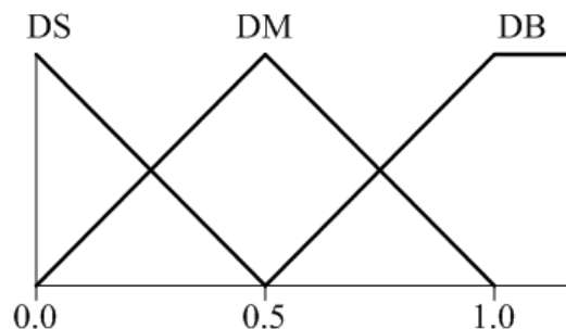
Figure 17. Membership function for each dynamic variable
