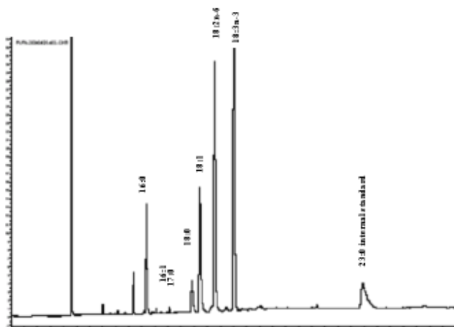
Figure 1. Chromatogram of fatty acid composition of jute seed oil analyzed with GC.
