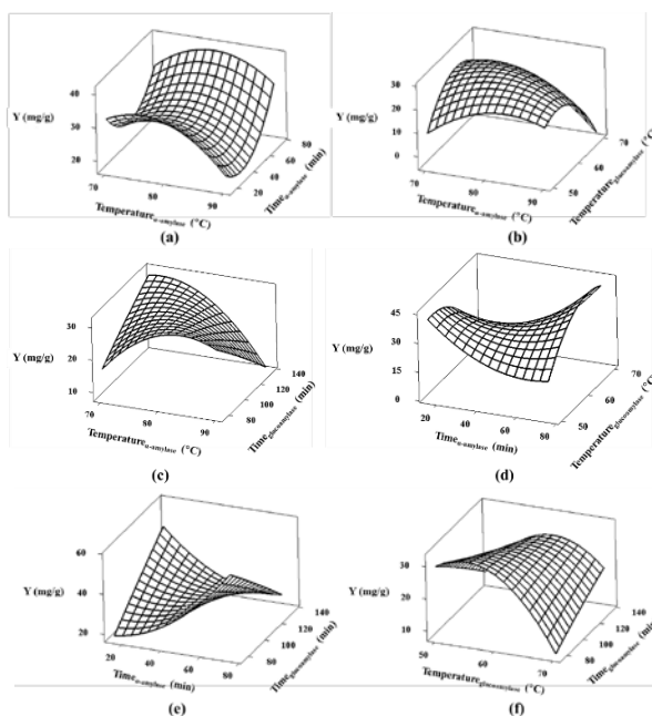
Figure 4. 3D Plots of reducing sugar yield ( Y ) for hydrolysis by \alpha -amylase and glucoamylase (a) hydrolysis temperature ( x_1 ) and time ( x_2 ) using \alpha -amylase; (b) hydrolysis temperature using \alpha -amylase and glucoamylase ( x_1 , x_3 ); (c) hydrolysis temperature using \alpha -amylase ( x_1 ) and hydrolysis time using glucoamylase ( x_4 ) (d) hydrolysis time using \alpha -amylase ( x_2 ) and hydrolysis temperature using glucoamylase ( x_3 ); (e) hydrolysis time using \alpha -amylase and glucoamylase ( x_2 , x_4 ); (f) hydrolysis temperature ( x_3 ) and time ( x_4 ) using glucoamylase.
