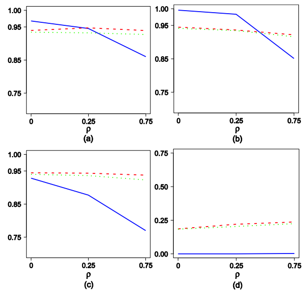
Figure 3. Plots of coverage probability of 95% confidence interval for the period \tau using DET (solid line), CLS (dashed line) and TS (dotted line) when the true model is song-sine and the fitted model is (a) one-sine, (b) song-sine and (c) two-sine with damping. Coverage probability plots for \nu in the two-sine with damping model are shown in (d).
