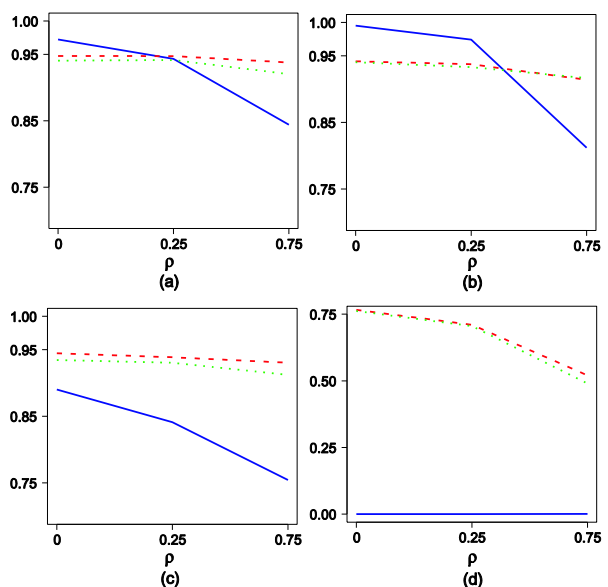
Figure 4. Plots of coverage probability of 95% confidence interval for the period \tau using DET (solid line), CLS (dashed line) and TS (dotted line) when the true model is two-sine with damping and the fitted model is (a) one-sine, (b) song-sine and (c) two-sine with damping. Coverage probability plots for \nu in the two-sine with damping model are shown in (d).
