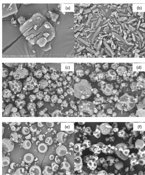
Figure 4. SEM photographs of \beta -CD (a), warfarin sodium (b) and spray dried powder of inclusion complexes between \beta -CD and warfarin sodium at mole ratio of 0.5:1 (c), 1:1 (d), 1.5:1 (e) and 2:1 (f).
