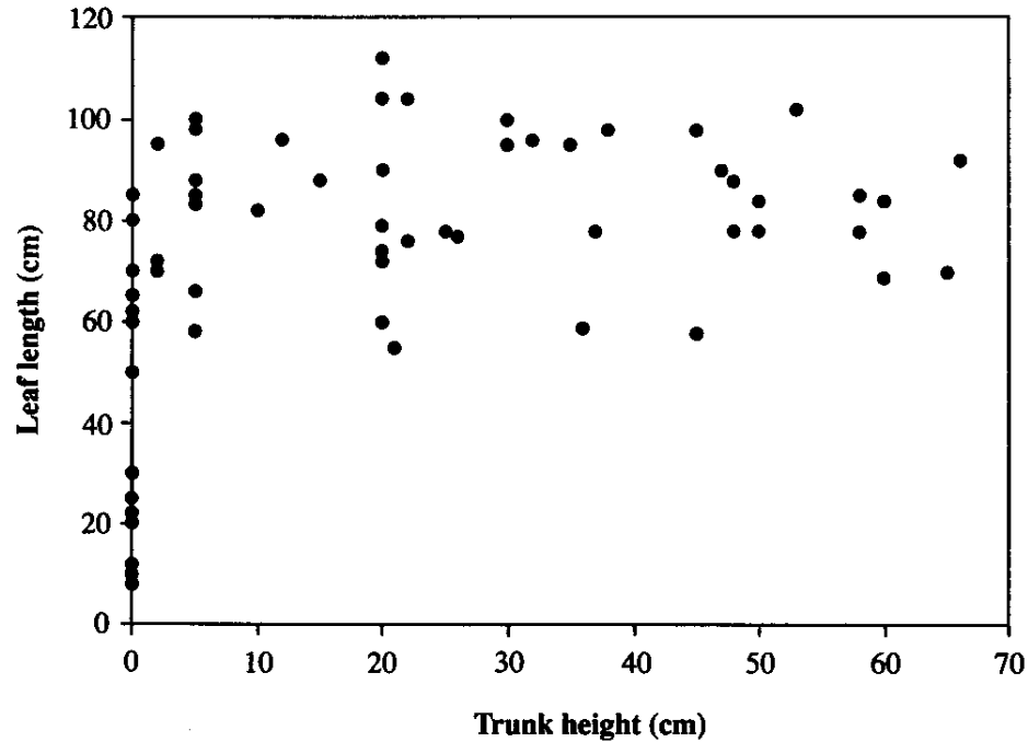
Figure 3. Relationship of mean leaf length to trunk height in Cycas siamensis at Sakaerat Environmental Research Station.
