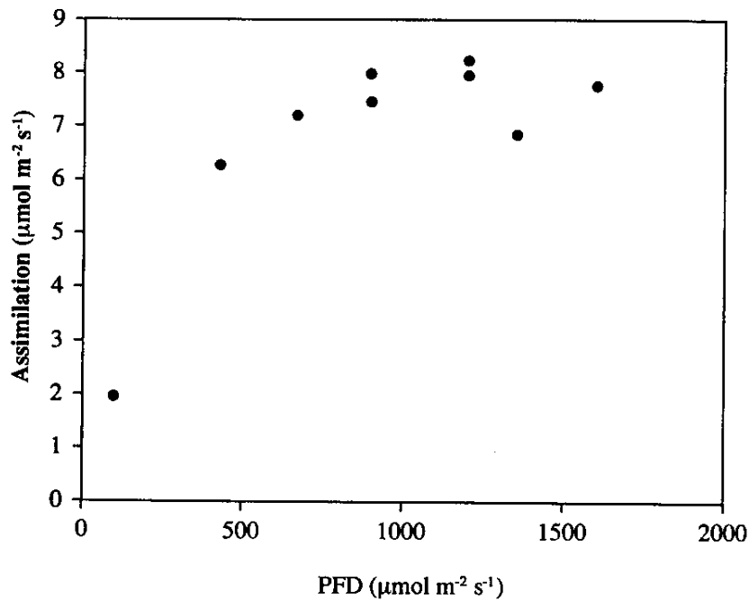
Figure 4. Light response curve for Cycas siamensis relating the rate of photosynthetic assimilation to photon flux density (PFD).
