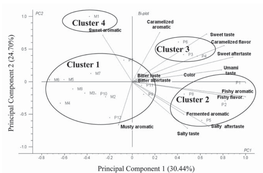
Figure 5 Biplot of the first two principal components for describing sensory attributes and grouping Thai fish sauces. P1-P12 are pure fish sauce samples and M1-M8 are mixed fish sauce samples.
