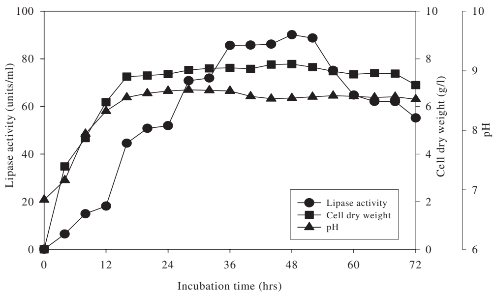
Figure 3 Time courses of growth, lipase production and pH of halotolerant Staphylococcus warneri PB233 in a 2-liters mini jar fermenter.
