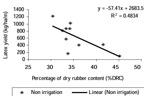
Figure 2 Correlation between latex and %DRC in non irrigation block.
